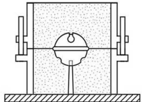
Fig 25 Stage 3 - The oddside box is removed and the bottom half of the bell is moulded.
