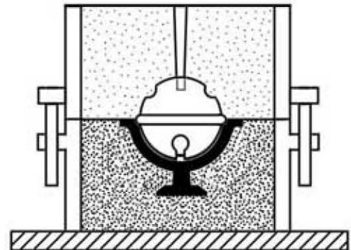
Fig. 24 Stage 2 - The pattern is placed in the oddside cup and the top half of the bell is moulded.
