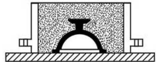
Fig. 22 Stage 1 - The oddside cup is set in a moulding box.
